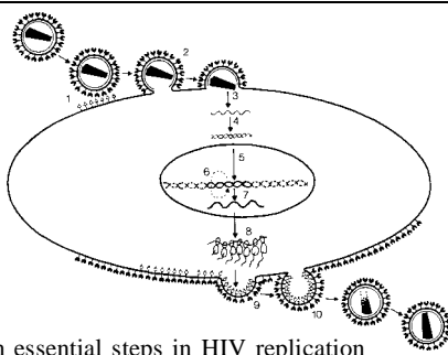
Ten essential steps in HIV replication
